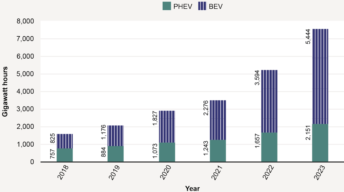
Figure 6-13 Estimated Electricity Use by Plug-In Vehicles: 2018–2023
