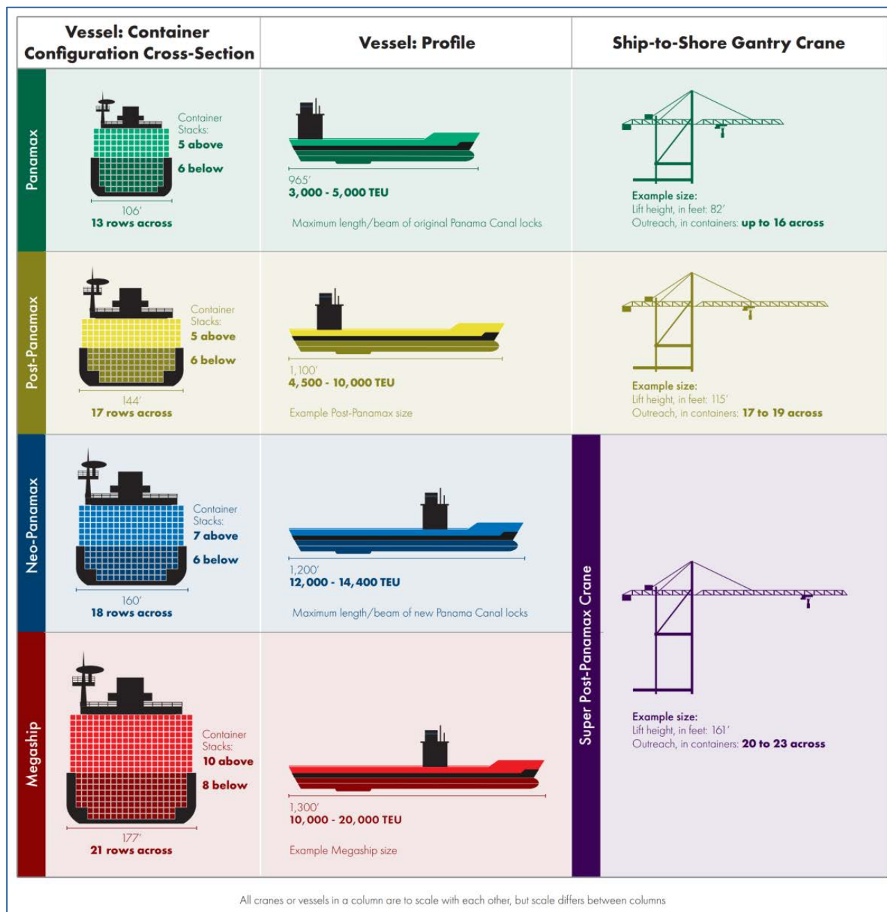
Figure 2-1: Increasing Vessel Size and its Impact on Port Infrastructure
